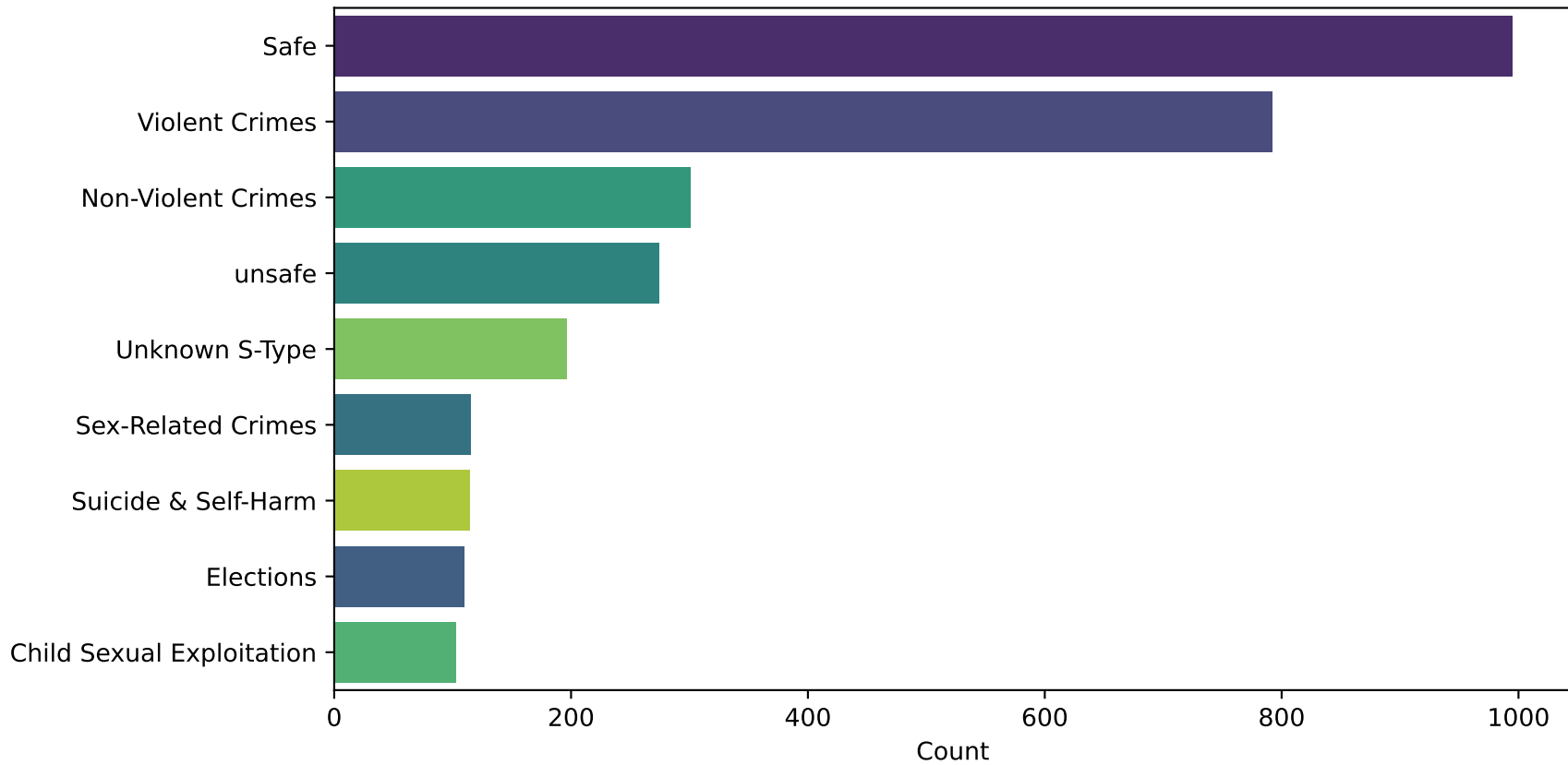
Class Distribution
